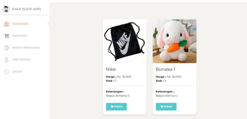
Gambar 5 Dashboard User.
