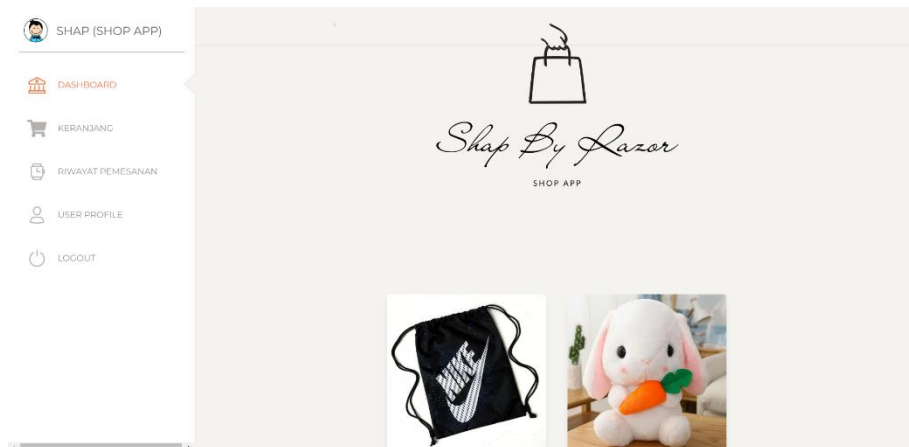
Gambar 18 Dashboard User.
